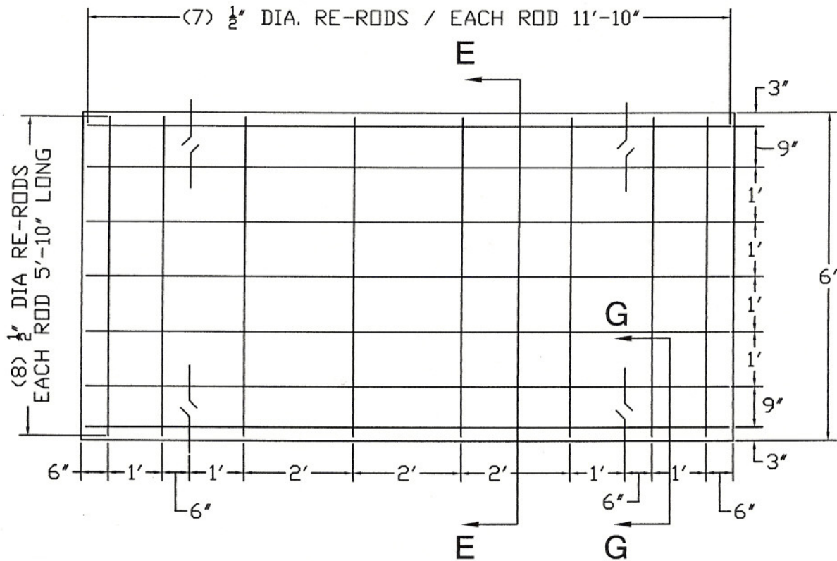
TOP VIEW
