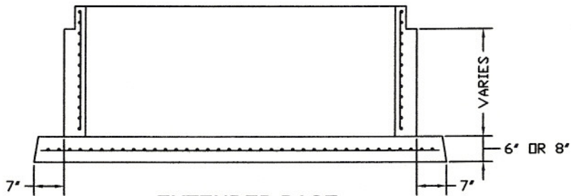
EXTENDED BASE
