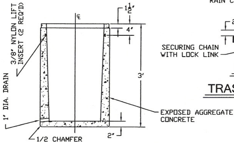
SECTION A-A TRASH RECEPTACLE
