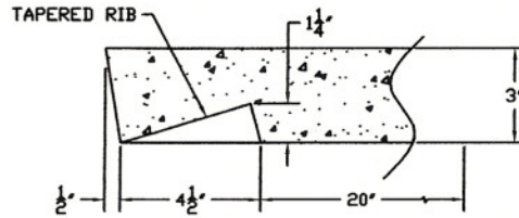
M.H. COVER END DETAIL
