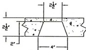
SECTION THRU 4" x 3" KNOCKOUT
