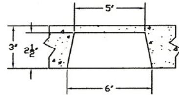
SECTION THRU 6" x 5" KNOCKOUT
