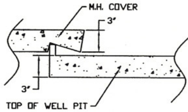
SECTION THRU MANHOLE SHOWING COVER IN PLACE
