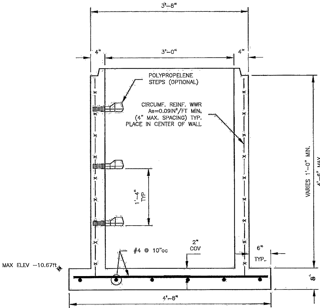
EXTENDED BASE SECTION VIEW
