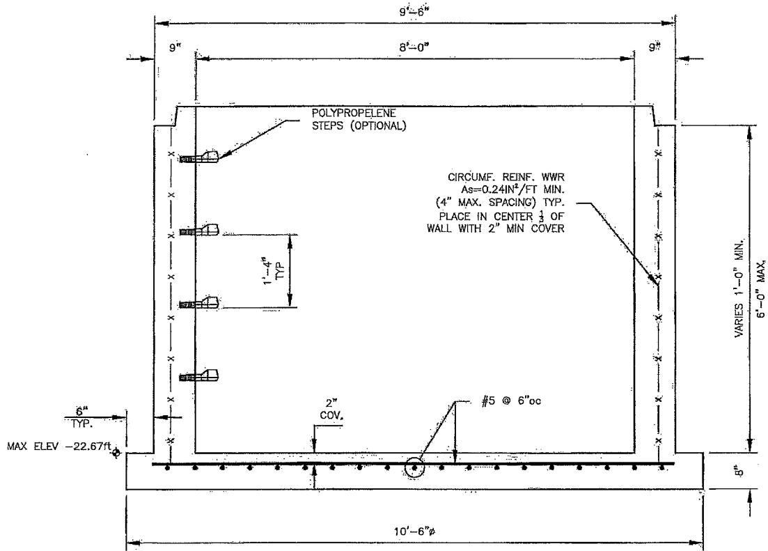
EXTENDED BASE SECTION VIEW
